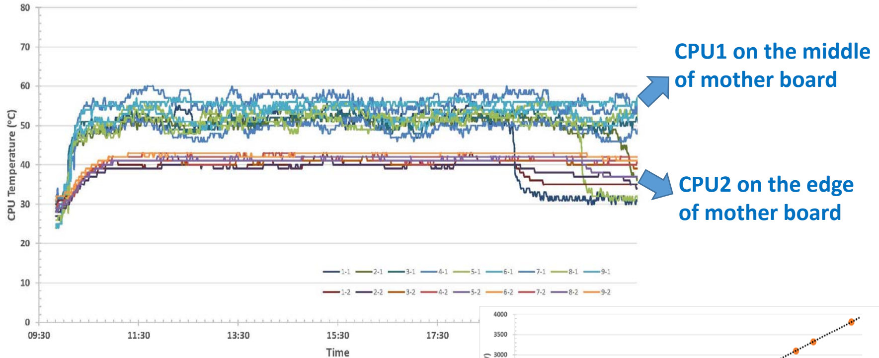
CPU Temperature of Fanless servers (Fully loaded with hyper-threading)
